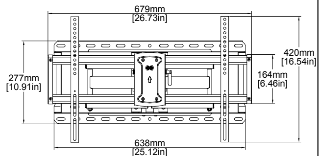
FULLY ASSEMBLED MOUNT
