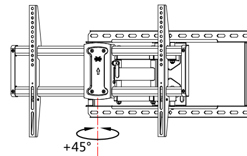
SIDE VIEW - EXTENDED
